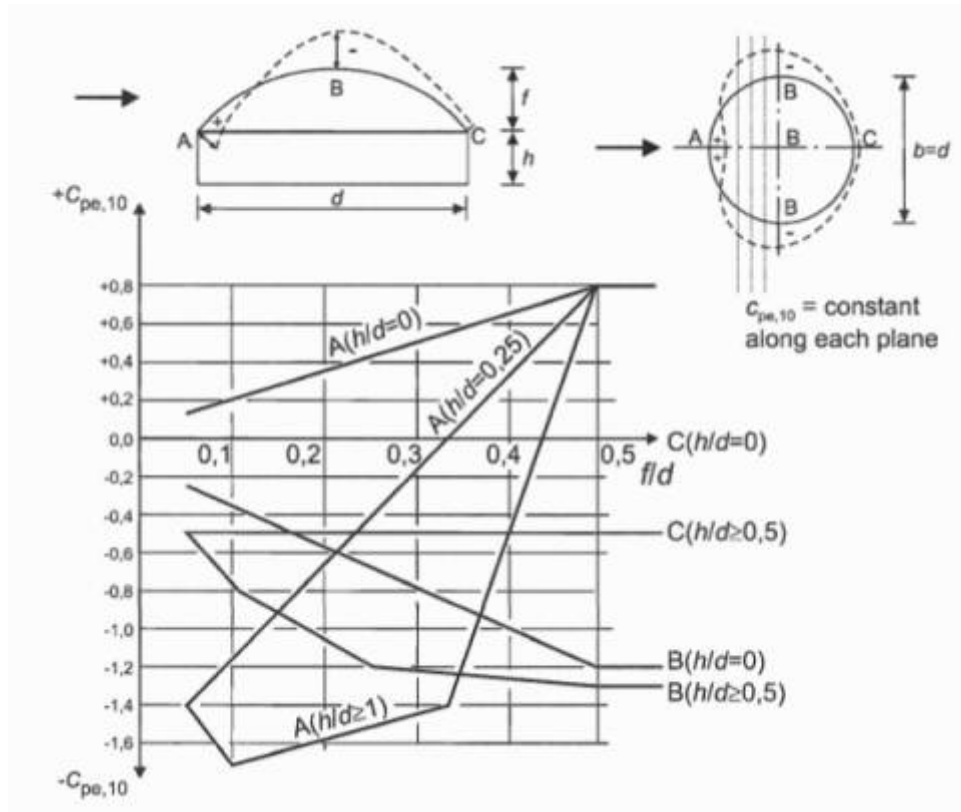
Figure 77: Shape coefficient for a dome shaped building
