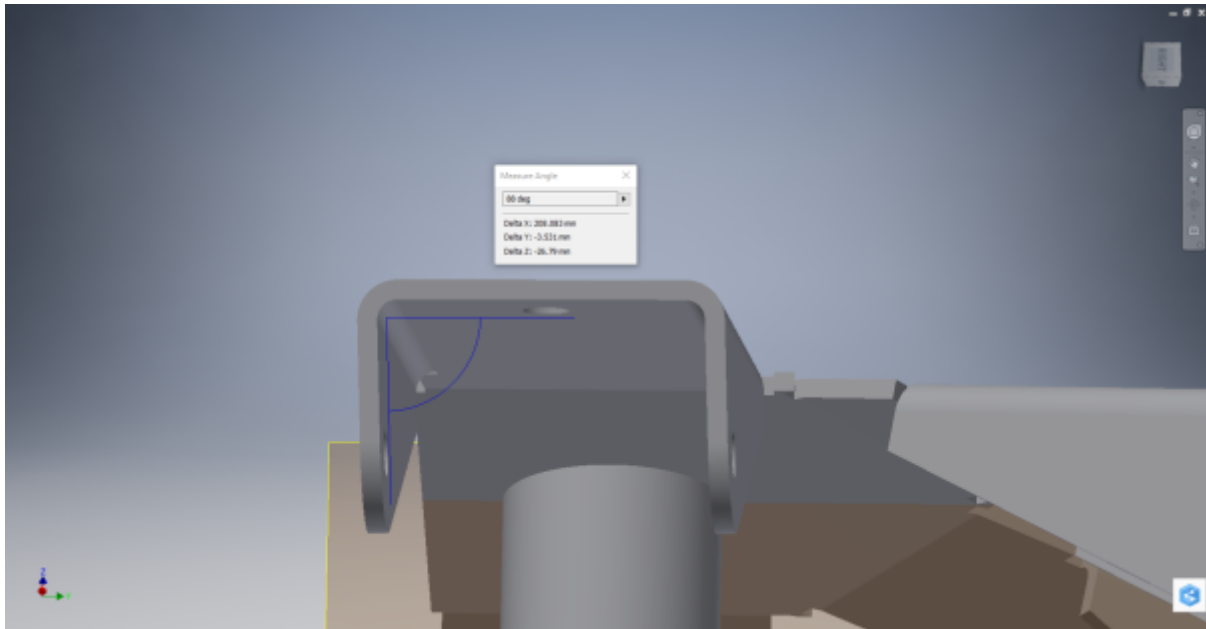
Figure 55: Side view of a 4 way connection
