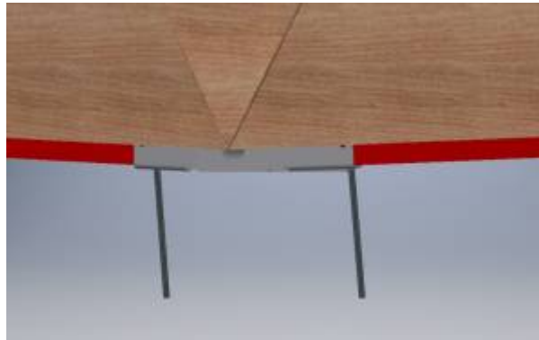
Figure 65: Connection node at the foundation
