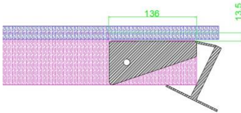
Figure 63: Cut at the end of a beam
