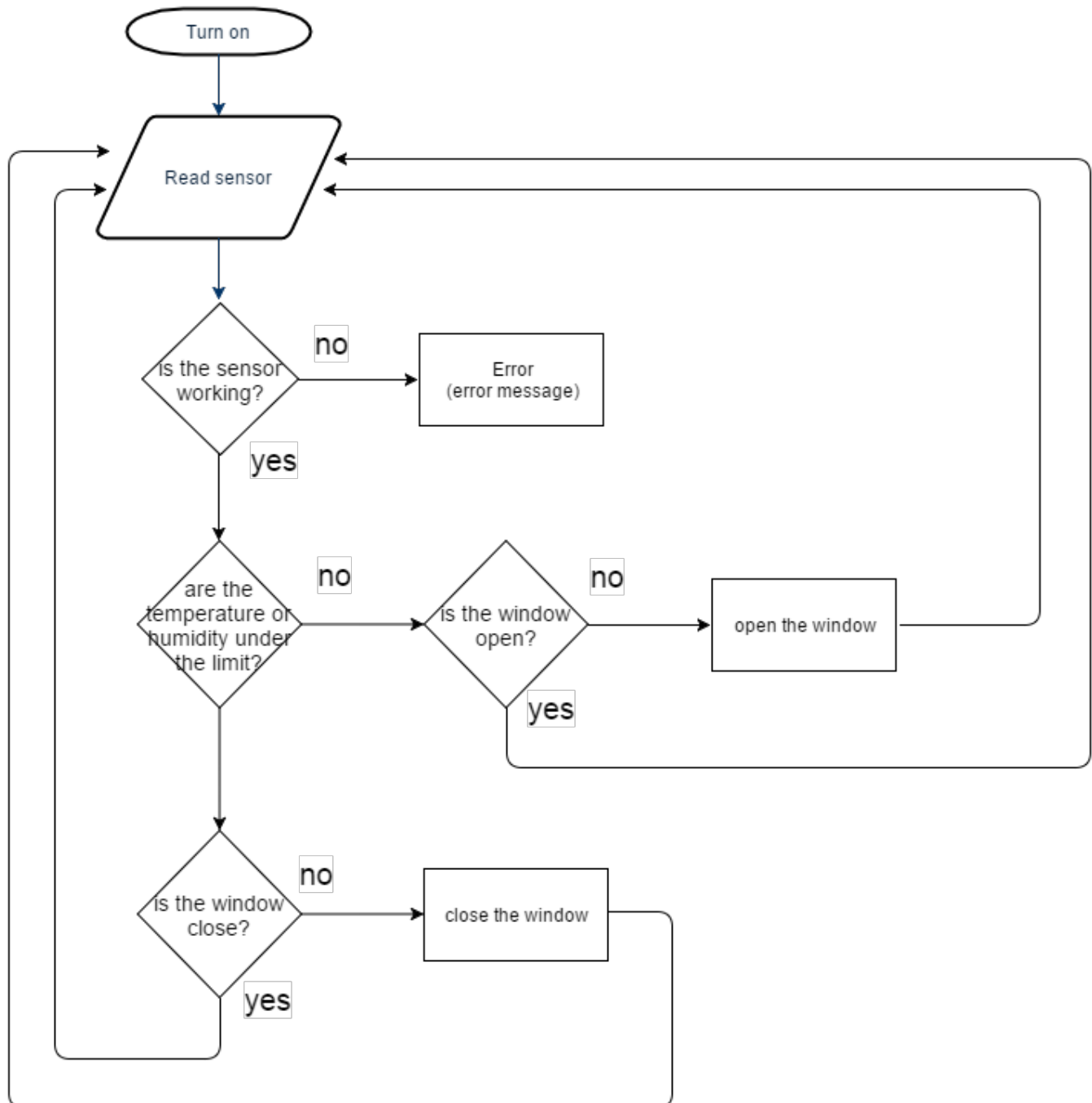
Figure 44: Flowchart for scale model
