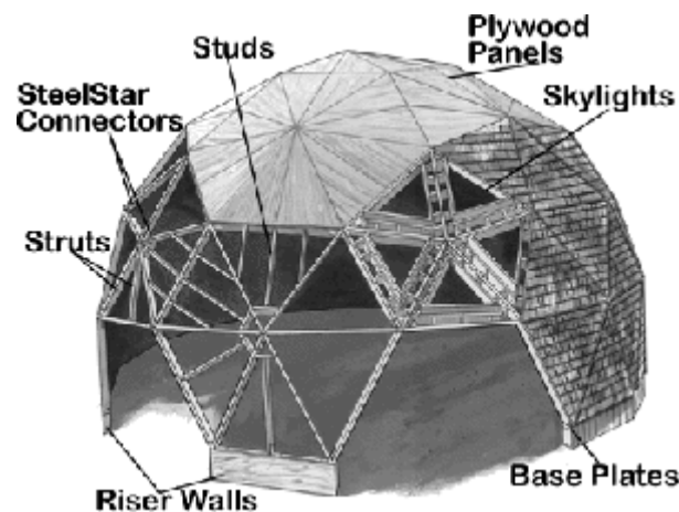
Figure 13: Structure Timberline Geodesic Dome [15]
