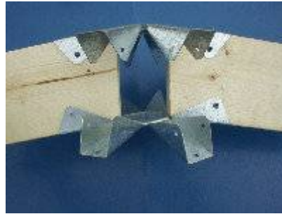
Figure 9: Use of the Simpson Strong-tie Gazebo [10]
