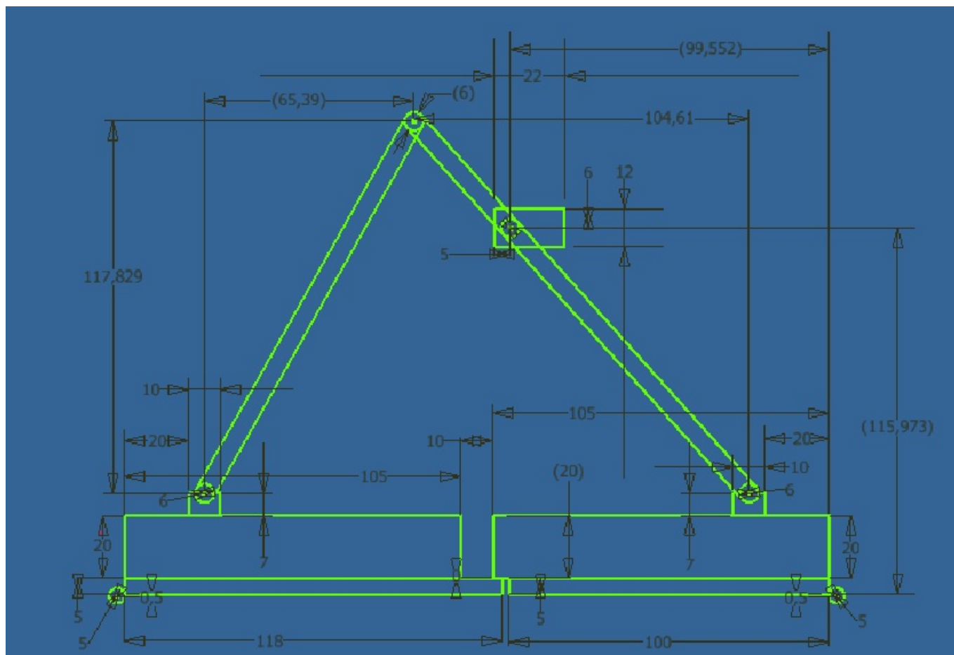
Figure 61: Closed door in top view
