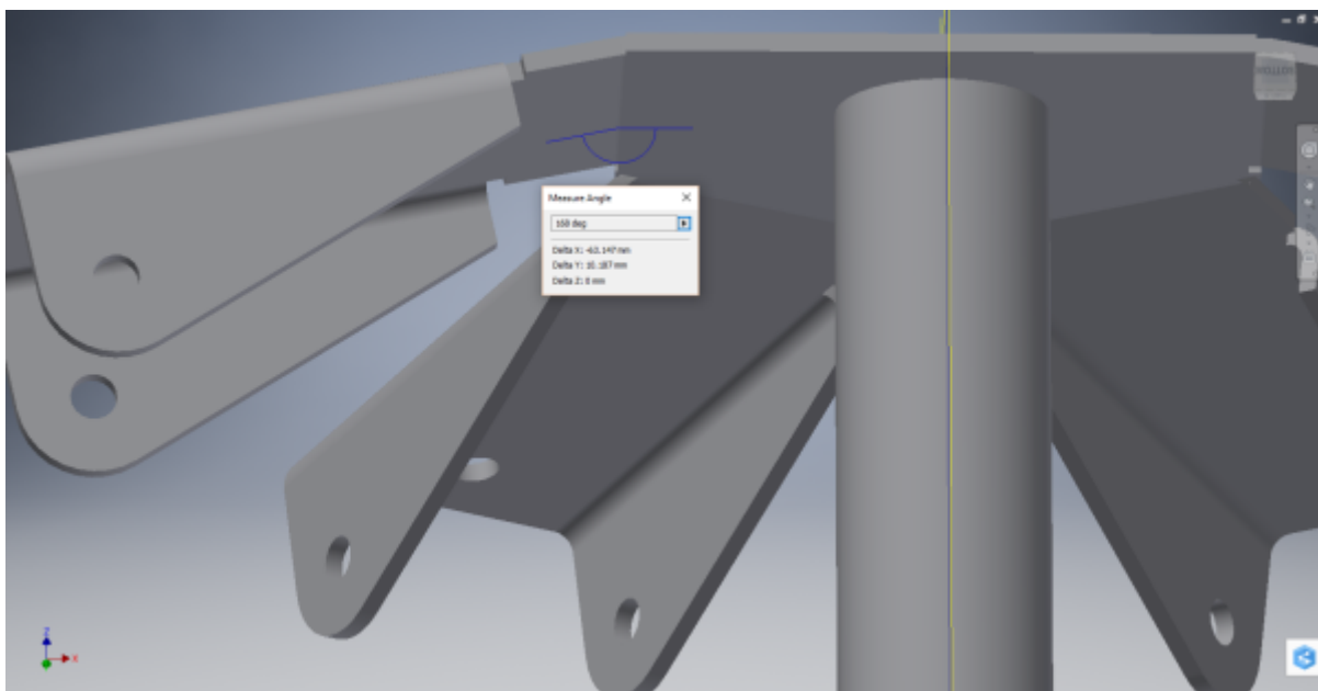
Figure 54: Side view of a 4 way connection
