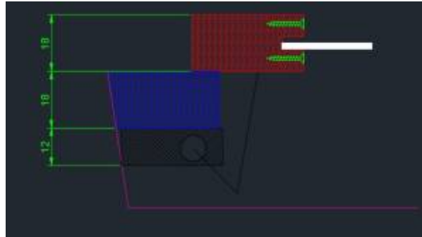
Figure 74: Position of the motor
