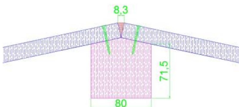
Figure 62: Connection of the panels to the beams
