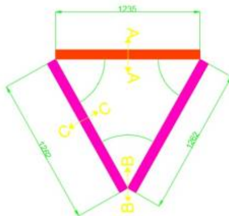
Figure 56: View of a triangle in which the window will be constructed
