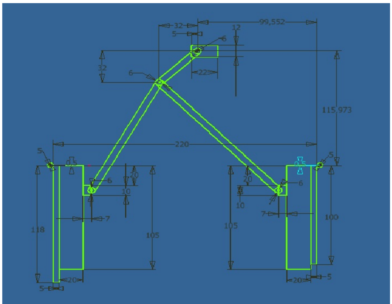
Figure 60: Opened door in top view
