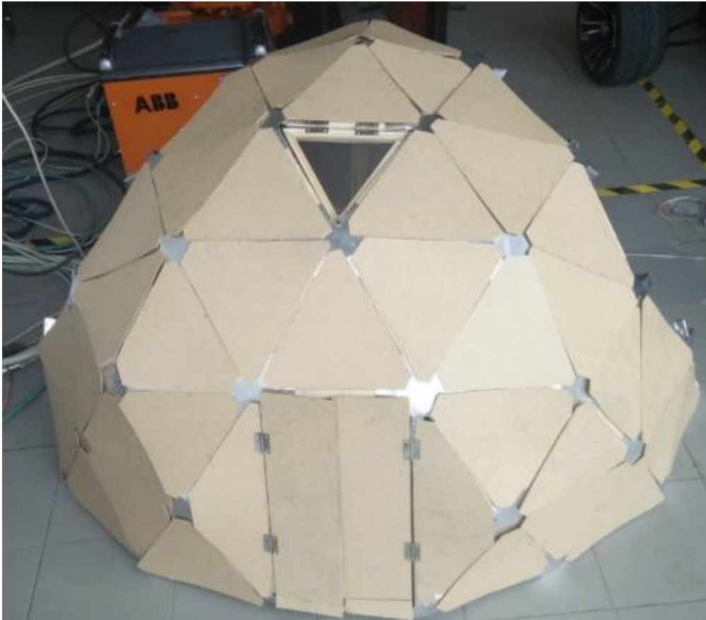
Figure 86: Prototype of the dome
