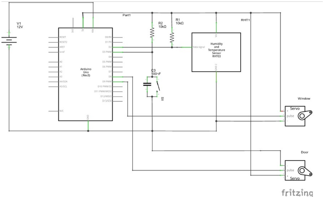
Figure 43: System schematics for scale model
