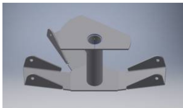
Figure 75: Concept of the connections between beams
