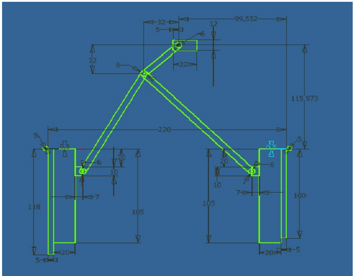
Figure 71: Opened door in top view
