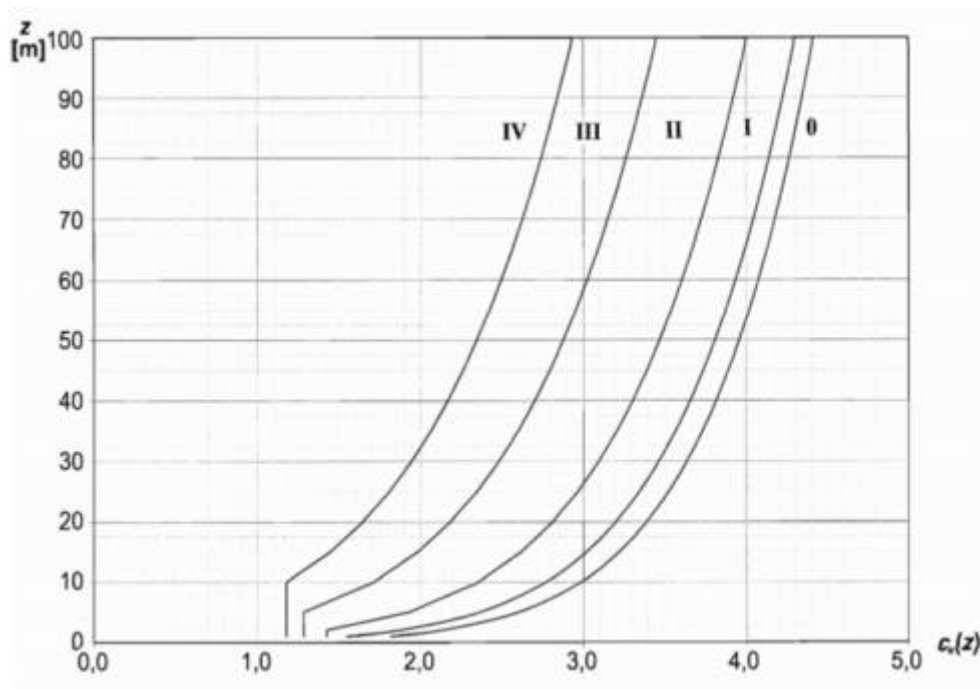
Figure 76: Terrain class and height of a building [63]
