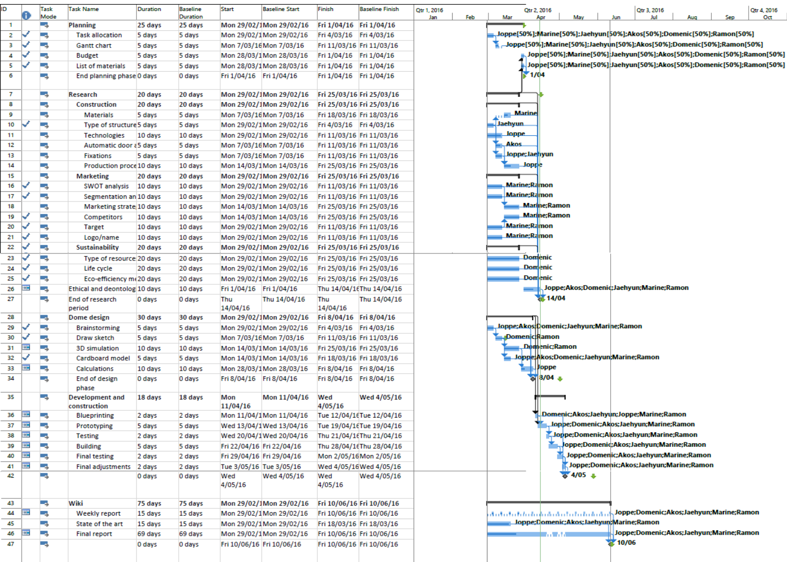
Figure 16: Gantt chart
