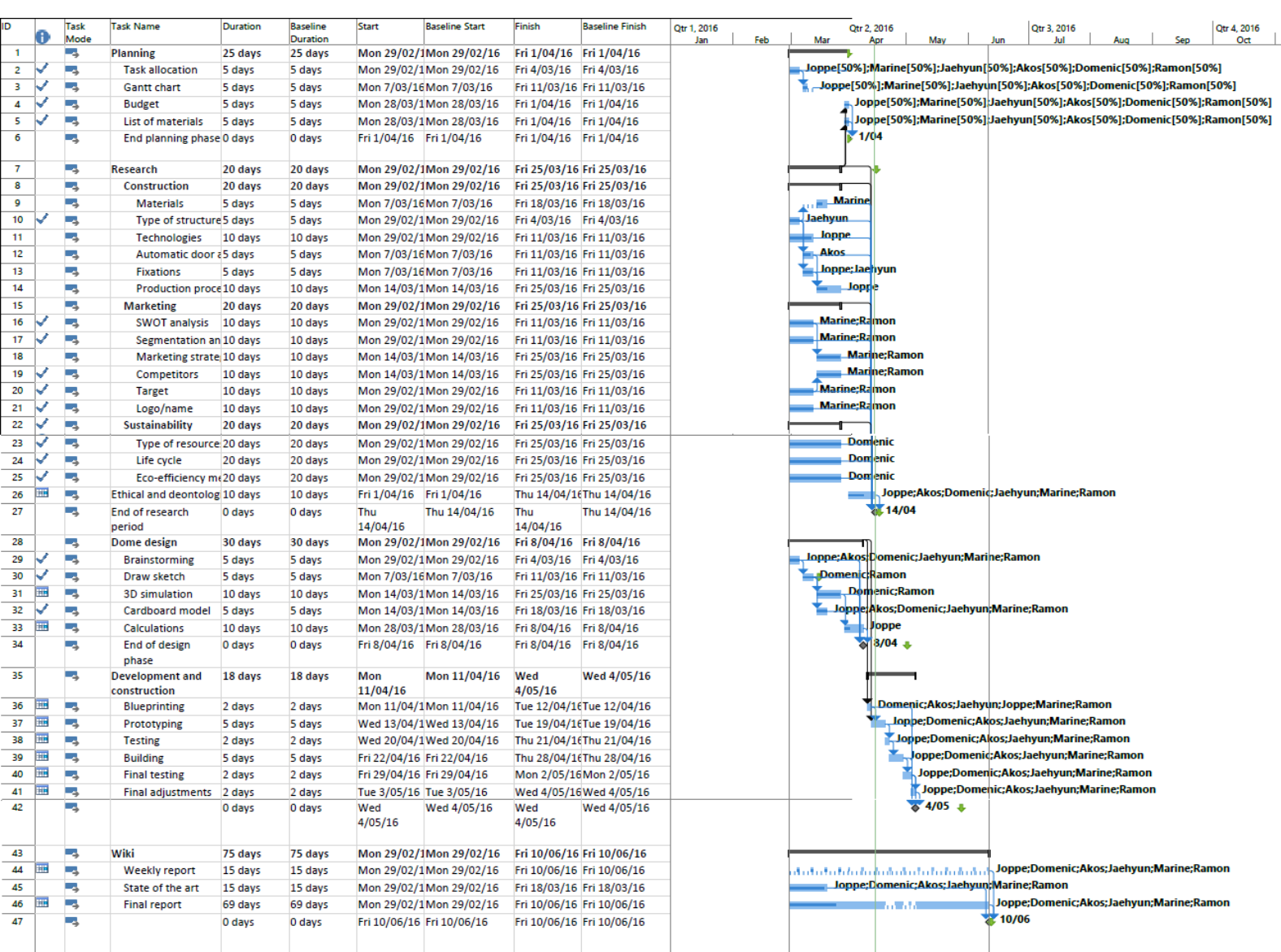
Figure 1: Gantt chart
