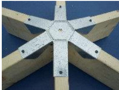
Figure 8: Simpson Strong-tie Gazebo Dome kits, 2016 [9]
