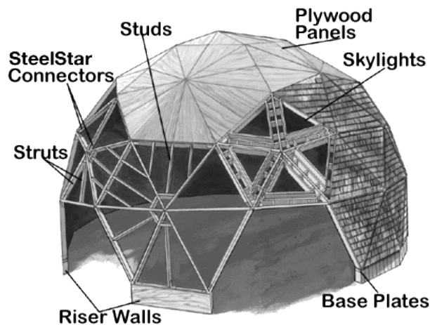
Figure 13: Structure Timberline Geodesic Dome Timberline Geodesics, 2014 [15]
