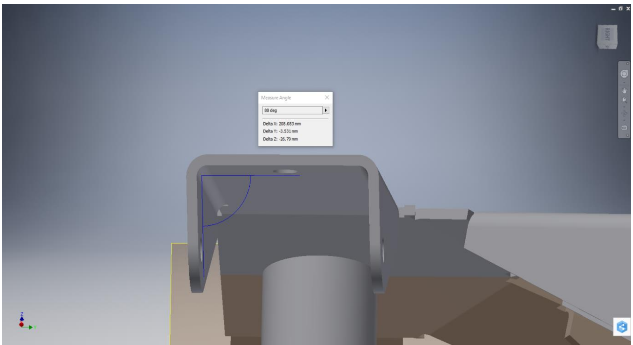
Figure 55: Side view of a 4 way connection
