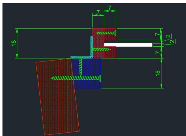
Figure 73: Section of the wood in the windows
