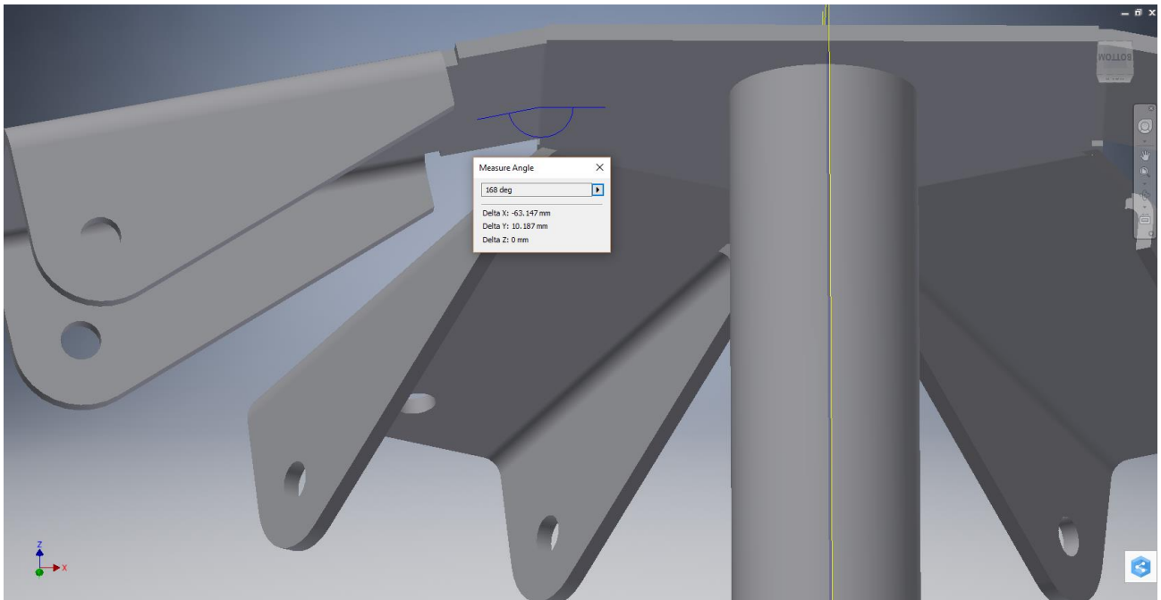
Figure 54: Side view of a 4 way connection
