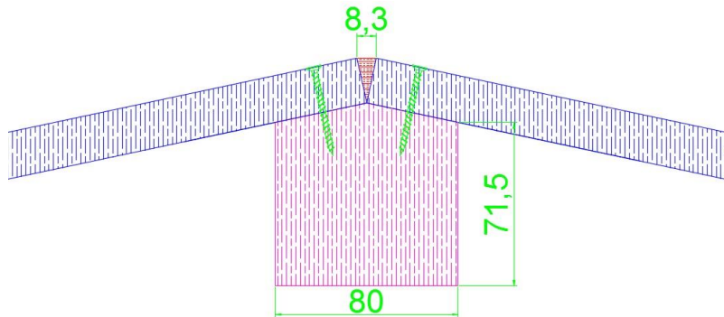
Figure 62: Connection of the panels to the beams
