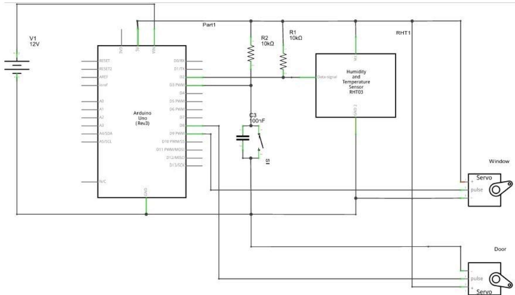
Figure 4 – System Schematics
